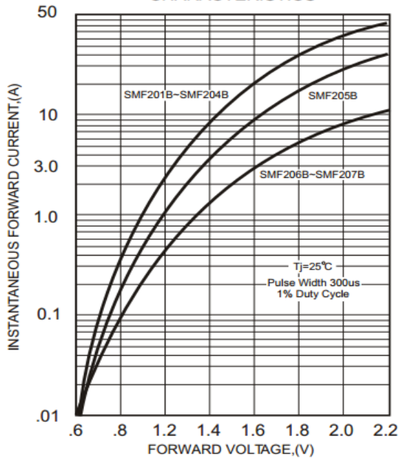
FIG.1-TYPICAL FORWARD CHARACTERISTICS
